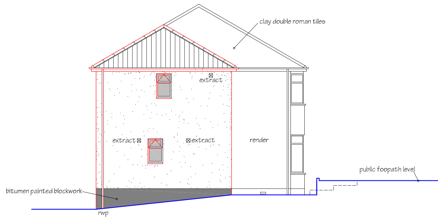
NORTH ELEVATION
