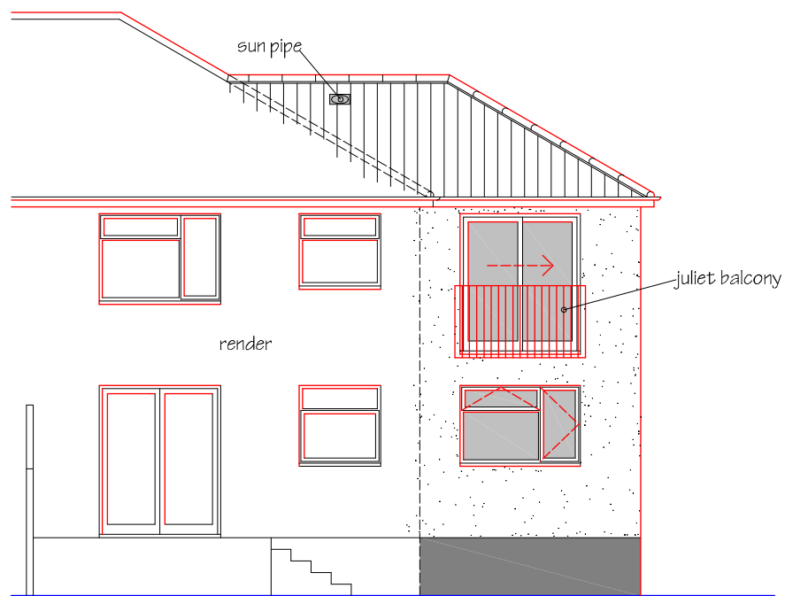
EAST ELEVATION
