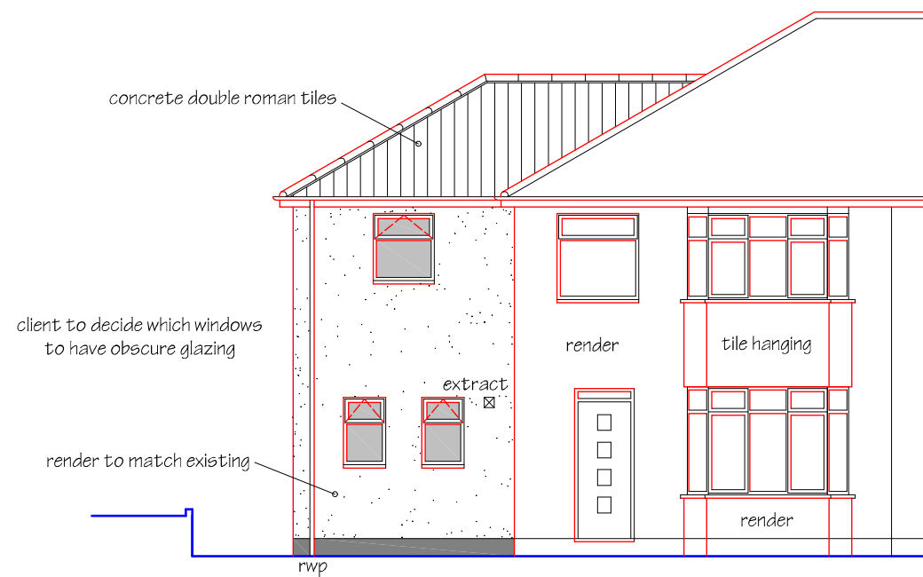
WEST ELEVATION
