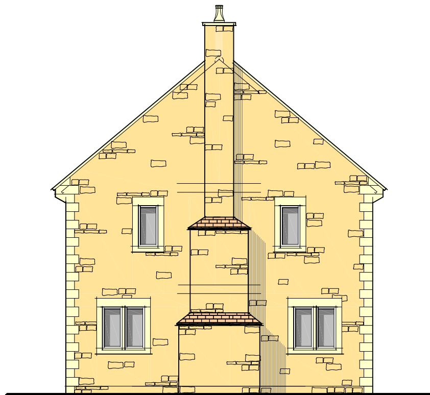
EAST ELEVATION
