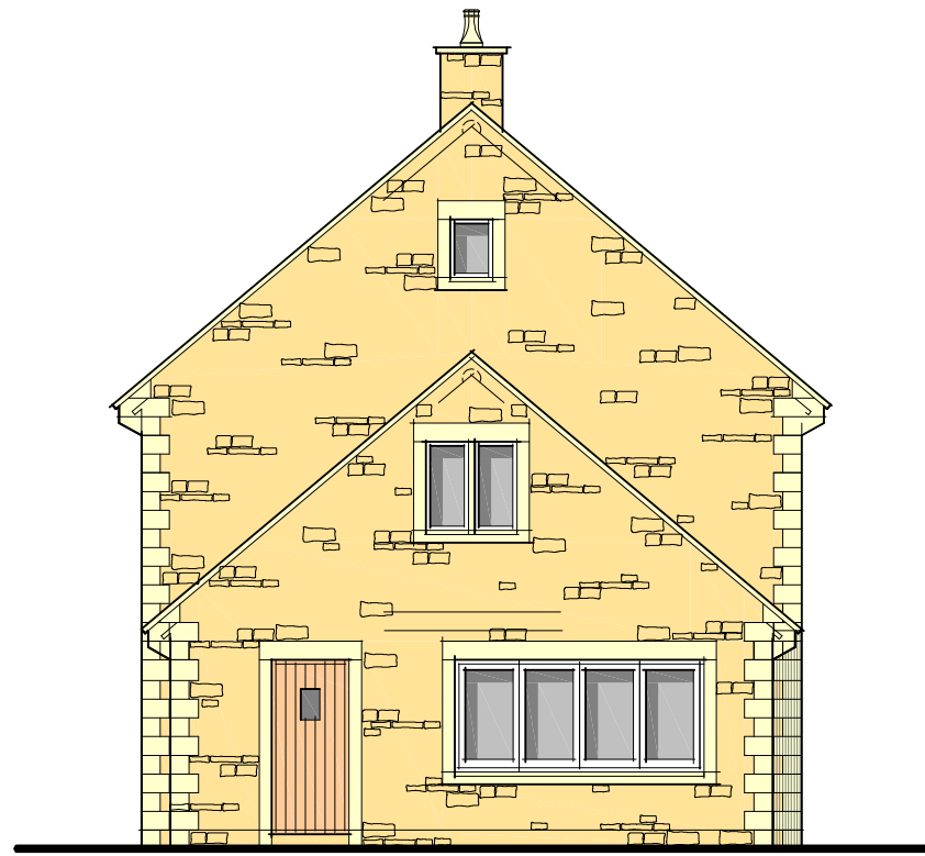
WEST ELEVATION
